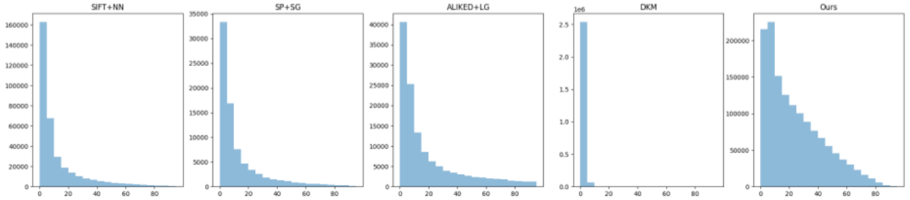
Figure 4. The distribution of track length using different feature matchers on IMC 2021 phototourism dataset [9]
