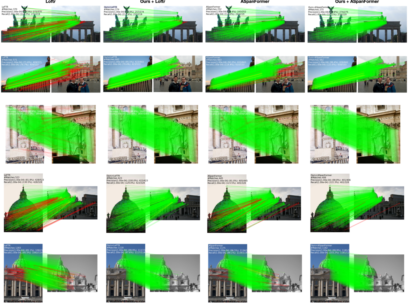
Figure 3. Qualitative Results on MegaDepth. Qualitative Comparison on MegaDepth [10]. The first column is LoFTR [17], the second column is Ours+LoFTR, the third is ASpanFormer and the fourth is Ours+ASpanFormer [2]. The green line indicates correct matches in which the symmetric epipolar error is less than 1e^{-4} , and the red line indicates wrong matches. By introducing the geometry constraints, one can see that the accuracy of matches is improved noticeably.
