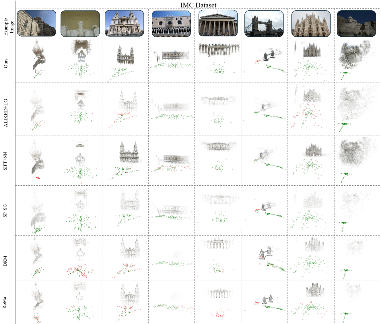
Figure 5. Qualitative results. Our method is qualitatively compared with other feature matching methods on IMC 2021 Phototourism Dataset[9]. Green cameras have less than 3^\circ absolute pose error, while red cameras have an error larger than 3^\circ .
